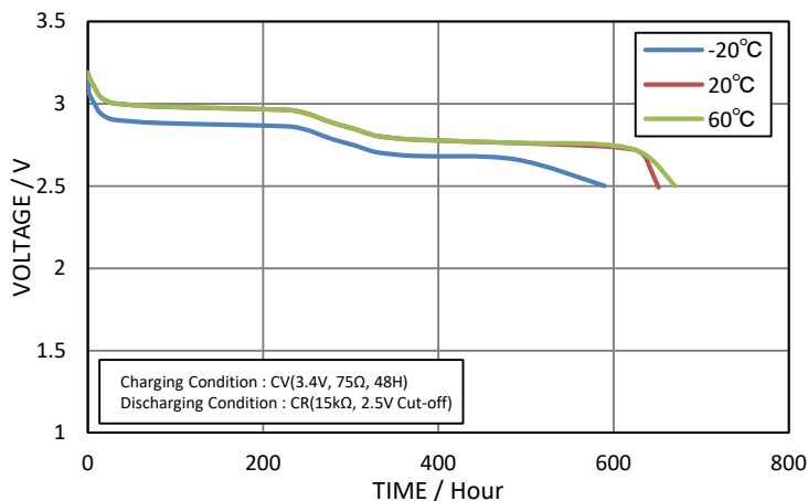
Discharging Characteristics
